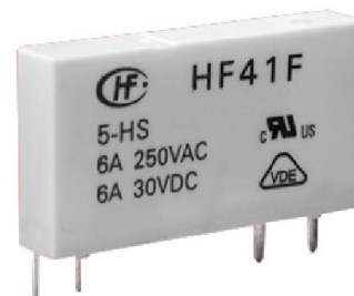
Relay HF41F
