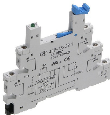
Relay Socket 41F
