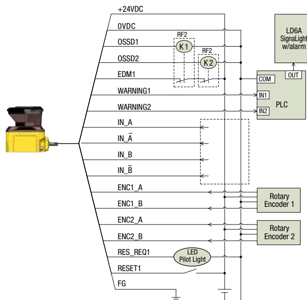
c) When switching 32 scanning areas using an encoder
